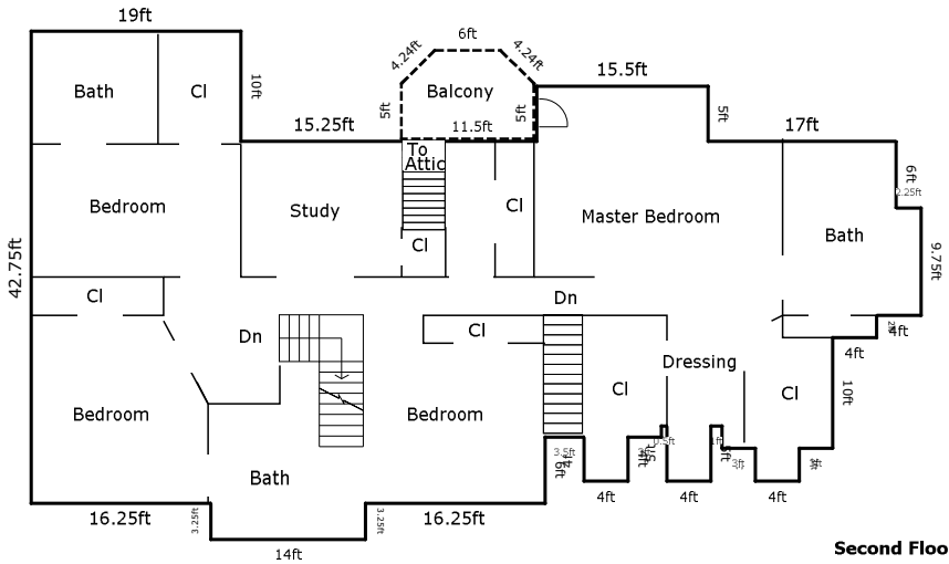
Second Floor [2704.38 Sq ft]
